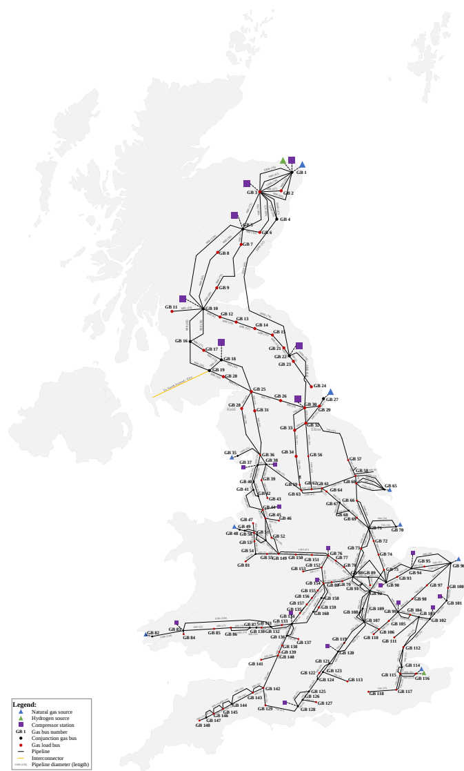
Fig. 14. Schematic diagram of the gas transmission system in the UK.
