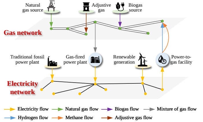
Fig. 1. Structure of the IEGS with the injections of alternative gases.
