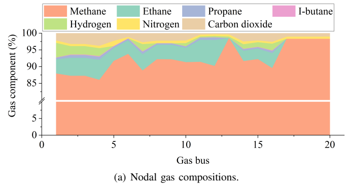
(a) Nodal gas compositions.
