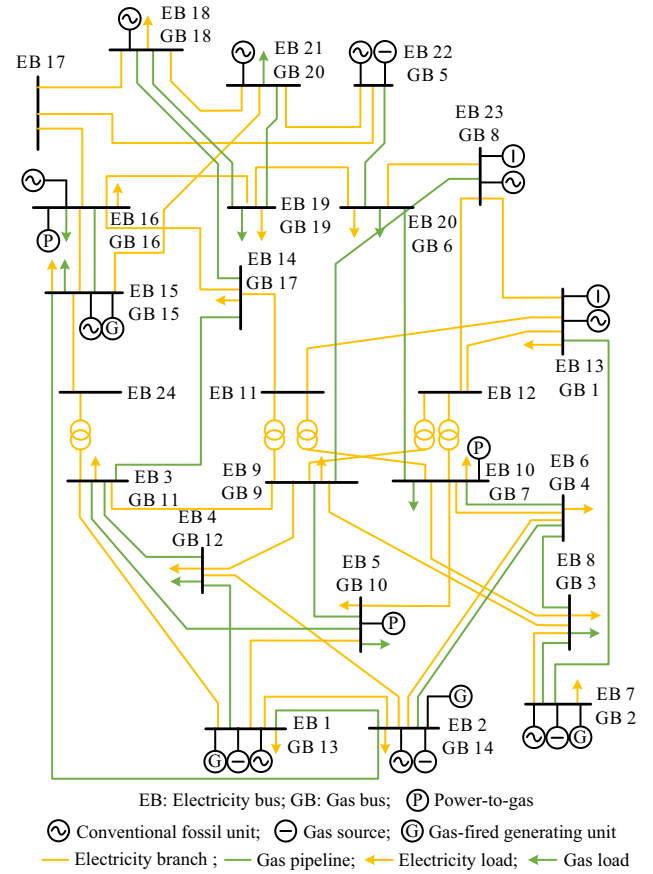
Fig. 4 Diagram for integrated IEEE RTS and Belgium natural gas transmission system
